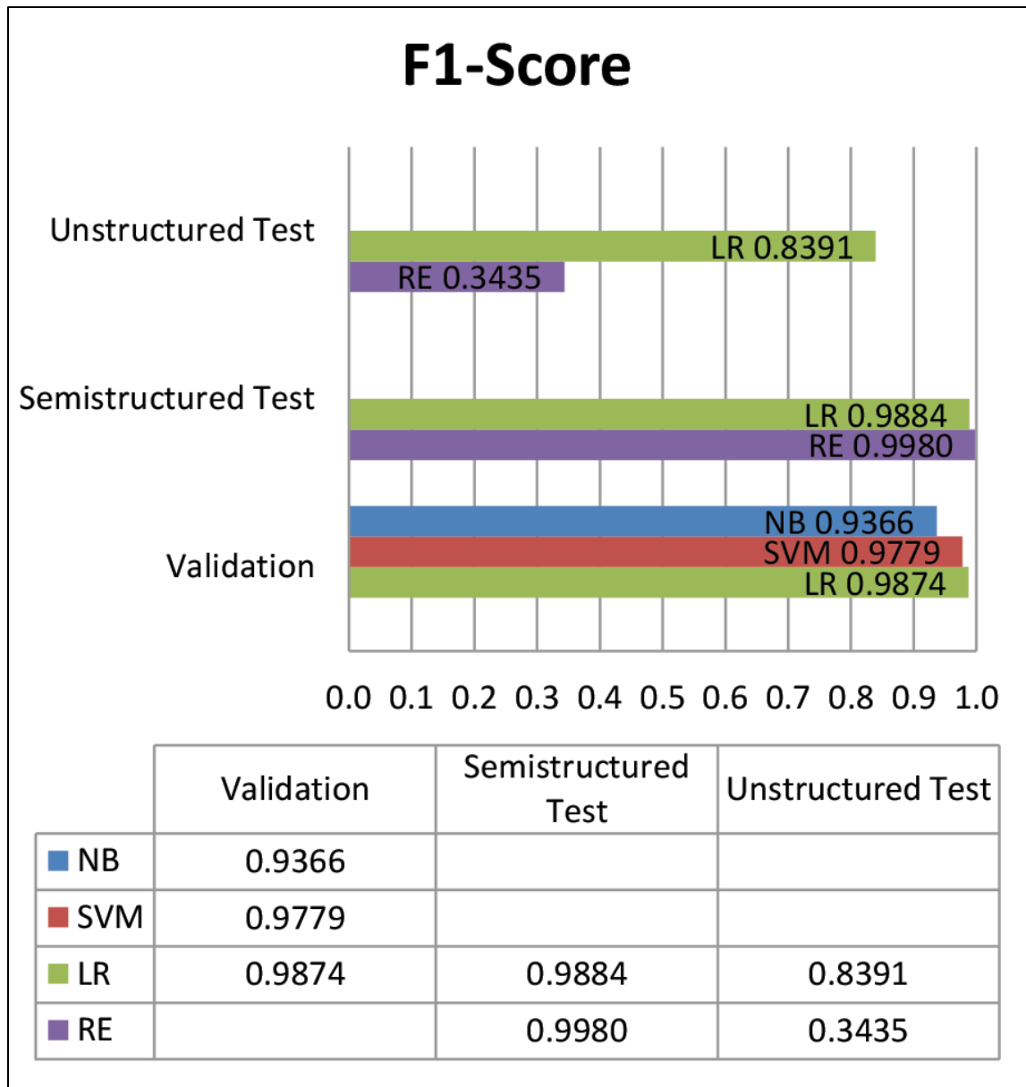
Figure 2.5: F1-Score Performance. All numerical values represent F1-scores.
