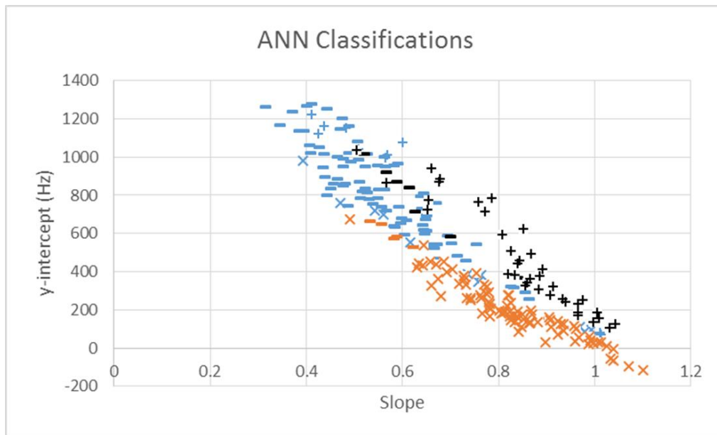
Figure 18: Dialect Java ANN
