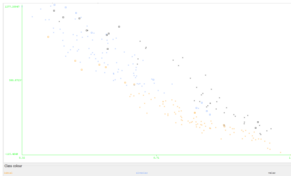
Figure 21: Dialect WEKA J48
