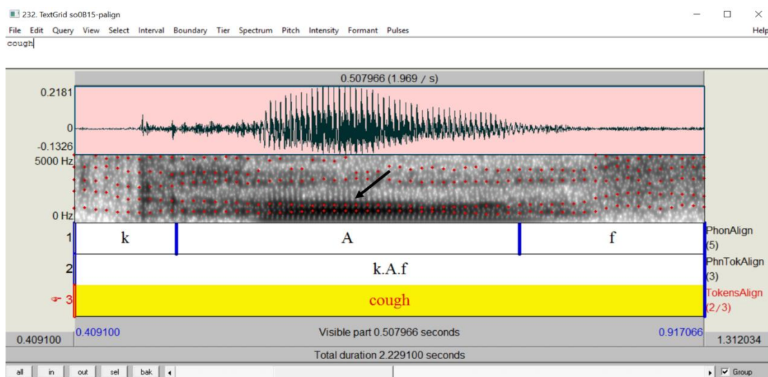
Figure 9: Monophthong Midpoint
