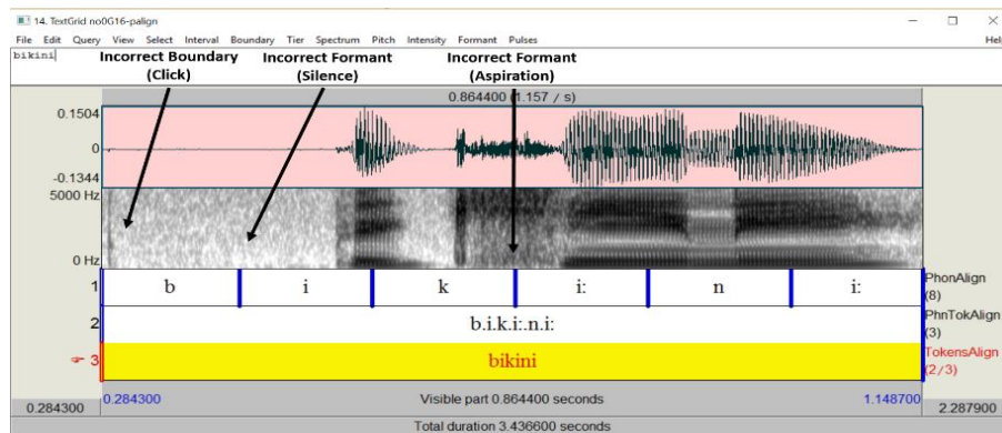
Figure 6: Alignment Error
