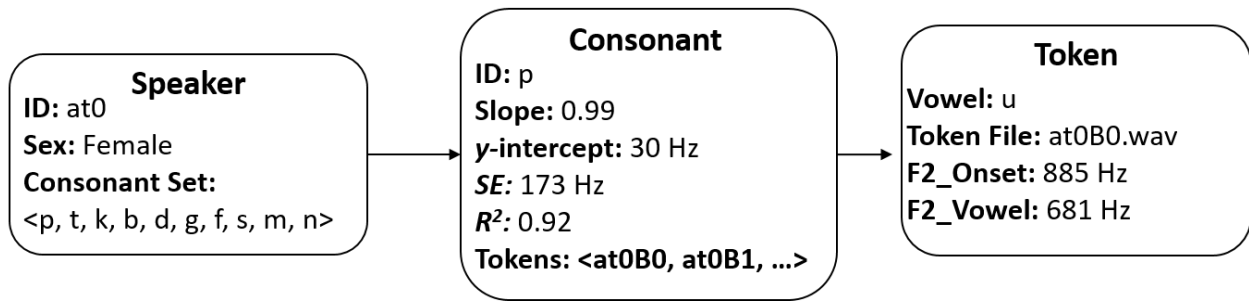
Figure 11: Java Classes
