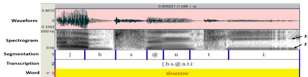
Figure 2: Formant Values
