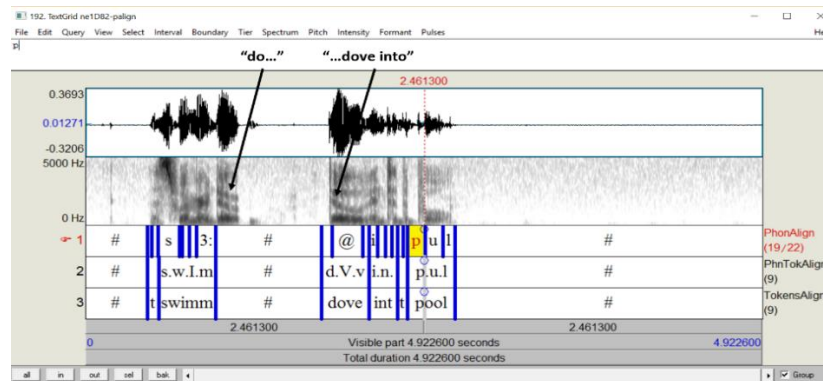
Figure 6: Alignment Error
