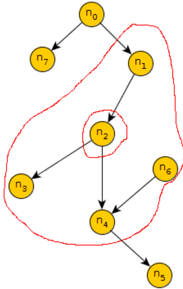
Figure 4.3: All the nodes between the two red boundaries make the Markov blanket for n_2 .
