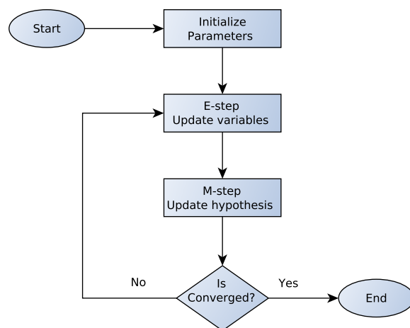
Figure 2.3: This flowchart illustrates the EM framework
