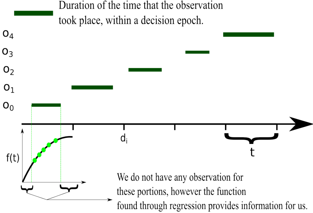
Figure 4.2: Illustration of f(t) . d_i shows the end of each decision epoch i . t is the continues time and each green bar shows potion of the decision epoch which the sound intensity samples are provided.
