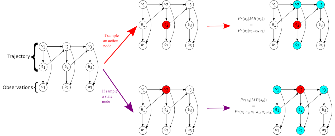
Figure 4.4: This image illustrates each step of the Gibbs sampling.
