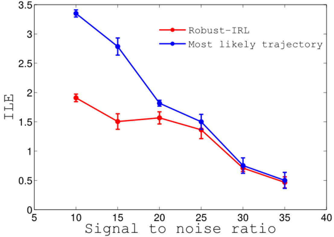
Figure 5.2: Performance evaluation of two methods for the learning drone reconnaissance routine simulation. ILE performance for the robust-IRL method and using most likely trajectory method. The horizontal axis shows the amount of noise added to the observation. As expected robust-IRL method has a better performance compare to the other method as the level of noise increases.
