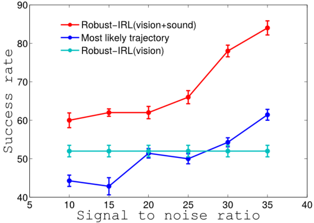
Figure 5.4: Performance evaluation of two methods on the Penetrating a patrol. This comparison is based on the successful runs. The robust-IRL method is evaluated using two different observation models. The horizontal axis shows the amount of noise added to the sound. As expected robust-IRL method has a better performance compare to the other method as the level of noise increases.
