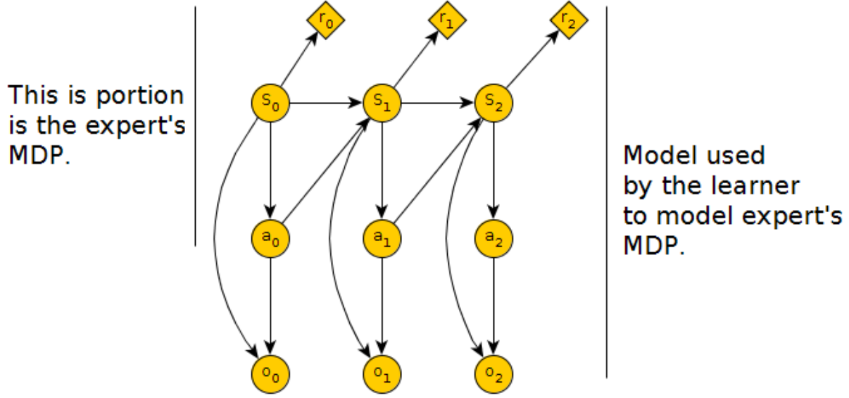
Figure 4.1: In hMDP the state and action are hidden from the learner but an observation of state and action is provided at each time step
