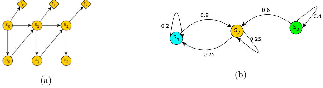
Figure 2.1: (a) An illustration of a MDP considering 3 horizons. s_i , a_i and r_i shows the state, action and reward of the agent at time step i . (b) A simple Markov chain with 3 state and 2 actions. The number on each edge indicates the probability of the transition.
