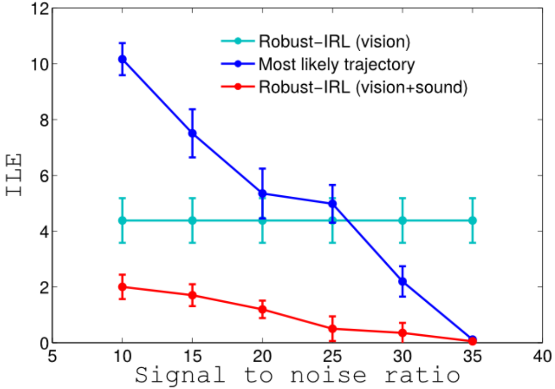
Figure 5.5: Performance evaluation of two methods on the penetrating a patrol simulation. ILE performance for Robust-IRL method and using most likely trajectory method. The robust-IRL method is evaluated using two different observation models. The horizontal axis shows the amount of noise added to the observation. As expected robust-IRL method has a better performance compare to the other method as the level of noise increases.
