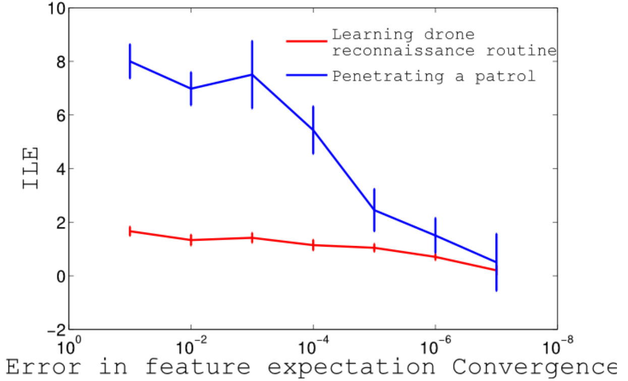
Figure 5.6: Performance evaluation of robust-IRL in two domains. The horizontal axis shows the convergence threshold in calculating the feature expectation in the E-step. The robust-IRL method is evaluated using two different observation models. Lower numbers means a tighter convergence condition. Lower ILE means higher accuracy.
