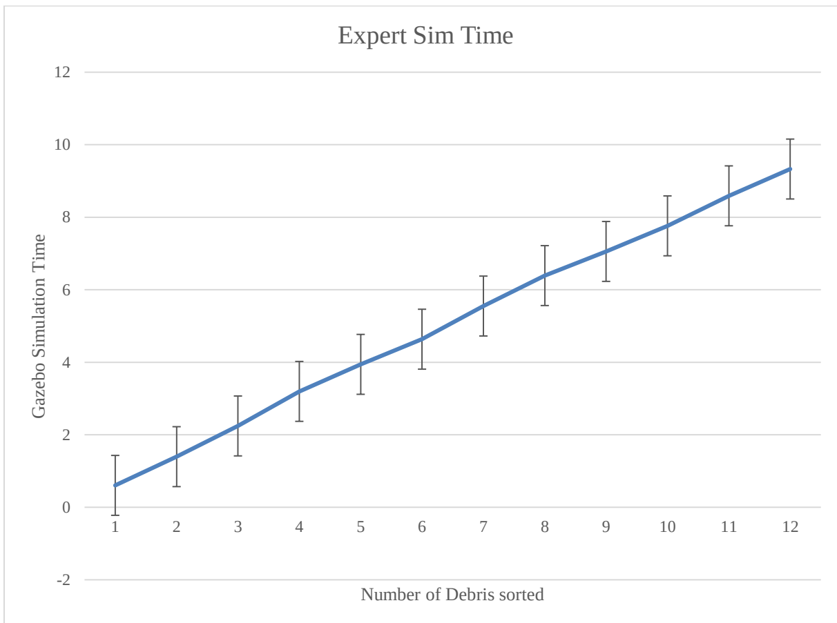
Figure 4.4 Sim Time vs Debris sorted for the Expert
