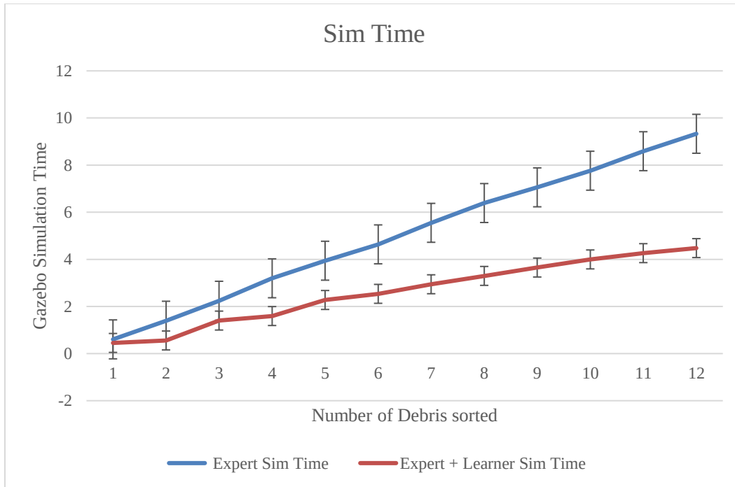
Figure 4.8 Sim Time vs Debris sorted for Single robot and Multi robot settings
