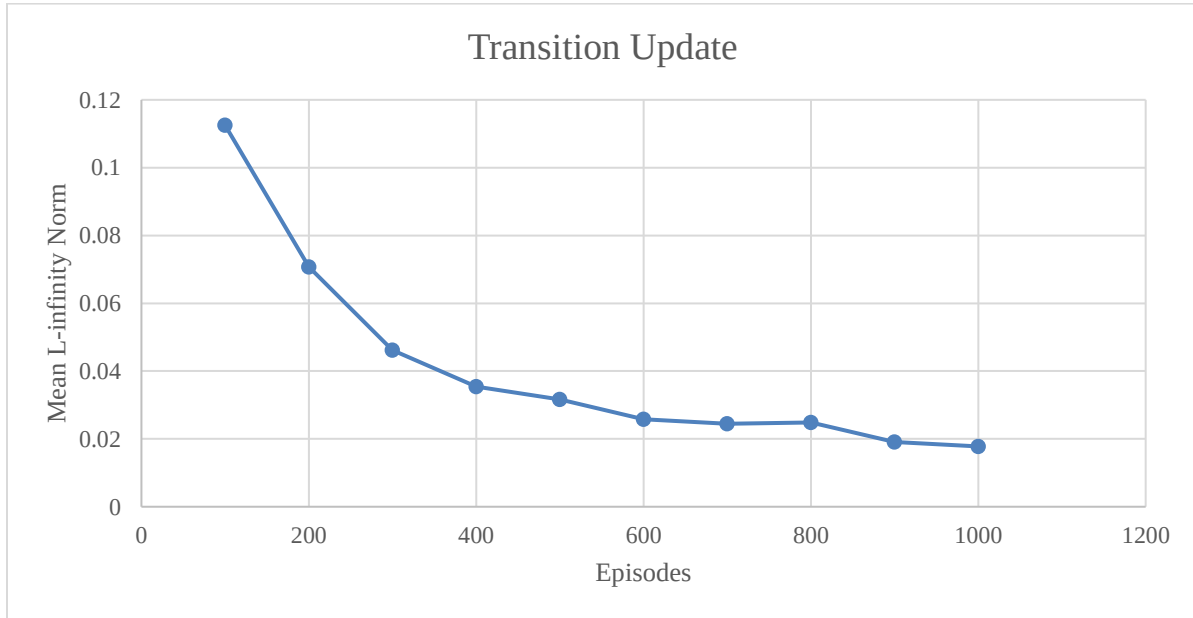
Figure 4.6 Count Vectors converging to the true state of the system
