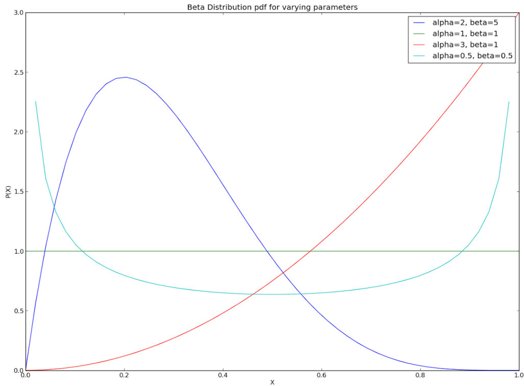
Figure 3.4 The above figure represents a beta distribution for different values of \alpha and \beta . The initial prior of (1, 1) represents a uniform prior distribution while successive pairs of (\alpha, \beta) map success and failures to their respective beta probability density function. As we increase the number of samples, this posterior probability density distribution starts to converge around the true state of the environment.
