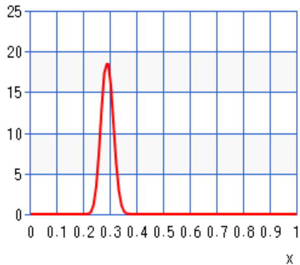
Figure 3.3 A Beta distribution with (\alpha, \beta) = (80 + 50, 220 + 100)
