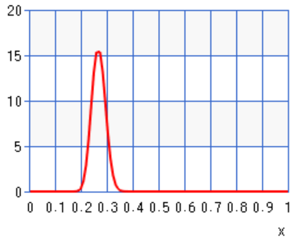
Figure 3.1 A Beta distribution with (\alpha, \beta) = (80, 220)
