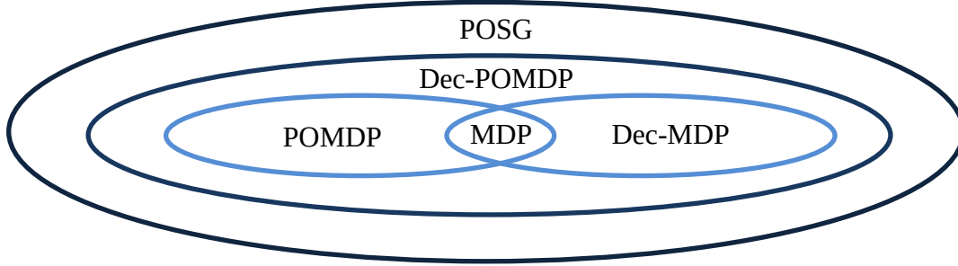
Figure 3.7 Types of Markovian Processes
