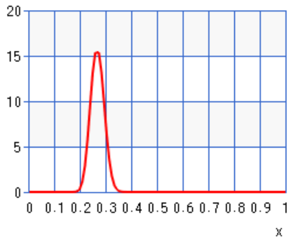
Figure 3.2 A Beta distribution with (\alpha, \beta) = (81, 220)
