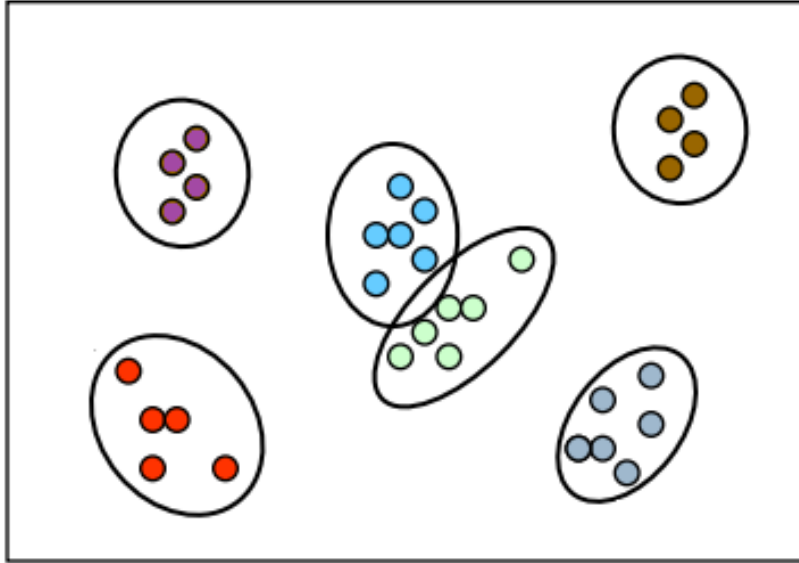
Figure 3.5 Example data set generated from a mixture of Gaussians
