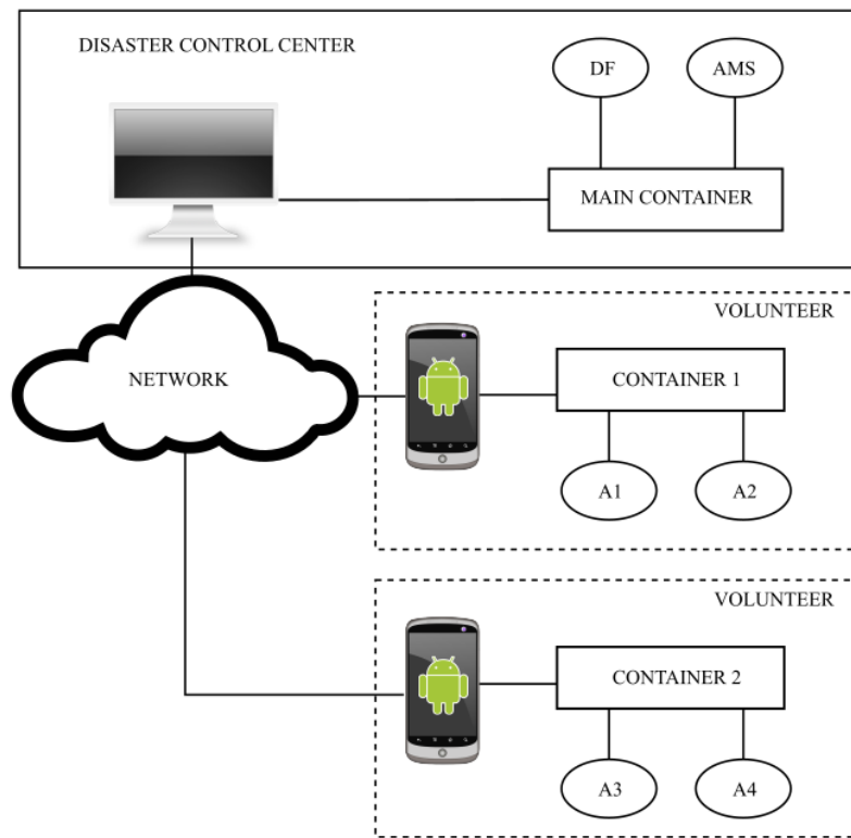
Figure 3.2: Configuration-I: Full containers on Android devices
