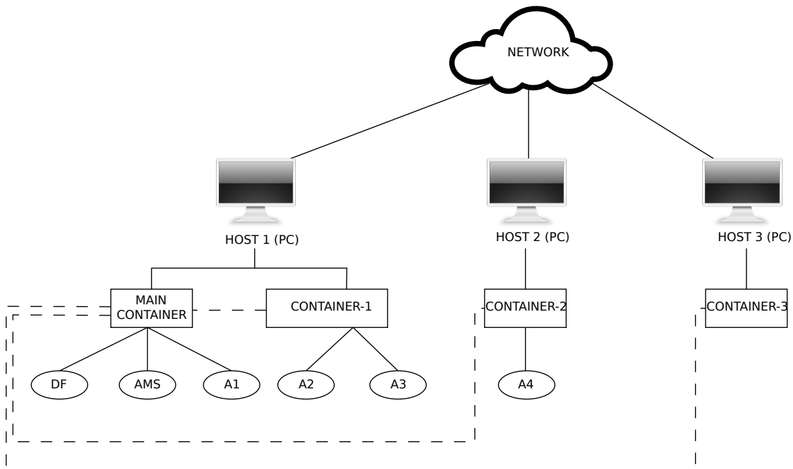
Figure 3.1: A JADE platform running on three different machines
